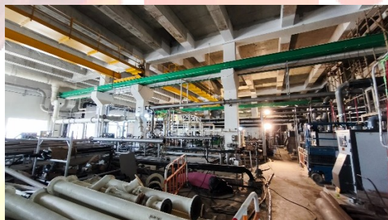
Cable Laying at Main Hall of Membrane Bio-reactor Treatment Facilities in Progress 薄膜生物反應處理大樓的電線接駁工程正在進行中
